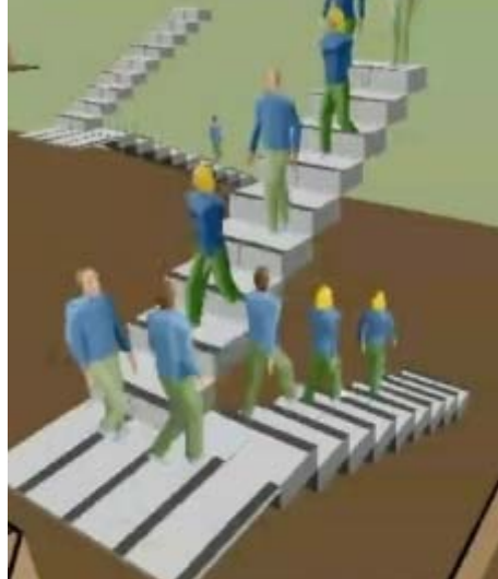
Figure 1: Predicting people movement down a stair (compliments of FSEG/EXODUS).
